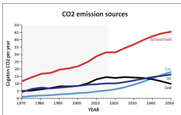
Figure 2.2.4: The rise in the direct use of oil and particularly gas, keeps pushing CO2 emissions despite cleaner electricity generation. The total use of fossil fuels in Faster is 18,000 Mtoe/year in 2050 relative to 12,000 Mtoe/year in Same .
