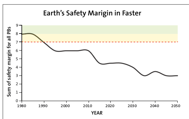
Figure 2.2.6: The Earth's safety margin is declining from 1980 all the way to 2050.
