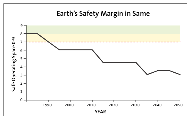
Figure 2.1.4 The Earth's safety margin as a sum of planetary boundaries (0= all in high risk, 9 = all safe).
